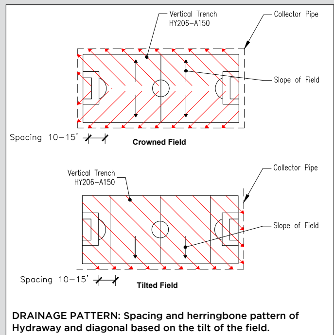
FIGURE 1. Typical baseball field layout of Hydraway.
